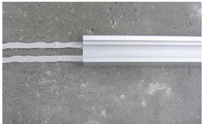
Bonding of aluminium runners on concrete with EGO SMP 808
